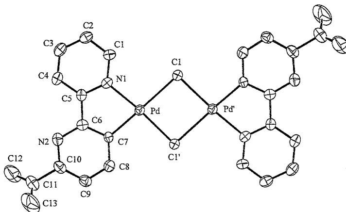
Fig 1. ORTEP view of [\text{PdCl}(\text{L}^1)]_2 , 1 . Primed atoms are related to unprimed ones by the symmetry operation -x, -y, 1-z . Ellipsoids are drawn at the 30% probability level
