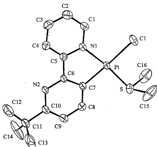
Fig. 2. ORTEP view of [\text{PtCl}(\text{L}^3)(\text{SMe}_2)] , 6 . Ellipsoids as in Fig. 1.
