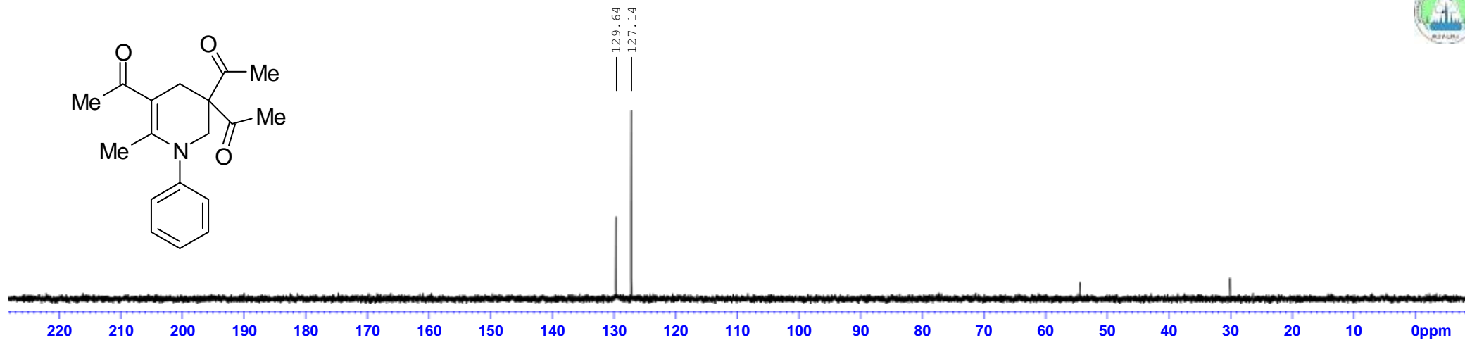
13C{1H}dept135 AV500
